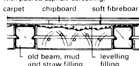
③ New floor covering (impact sound insulation)
